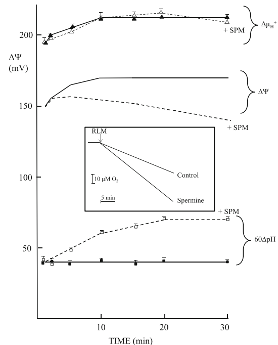
Fig. 3 Changes in \Delta\Psi and 60\Delta pH during spermine (SPM) transport. RLM (1 mg of mitochondrial protein/ml) were incubated in the experimental conditions as in Fig. 1 in the presence of 1 mM Pi. 1 mM spermine was added. \Delta\Psi was measured as in Fig. 2. \Delta pH was detected by using DMO distribution across the membrane (Rottenberg 1979) at the times indicated by the experimental points. \Delta\mu_{H^+}^+ was calculated by the equation \Delta\mu_{H^+}^+ = 60\Delta pH + \Delta\Psi by extrapolating the ordinate axis and the \Delta\Psi values were obtained with the TPP + electrode at the same times as for 60\Delta pH determinations. In this regard the \Delta\Psi scale has been linearized. In the inset, oxygen uptake was determined by the Clark electrode
